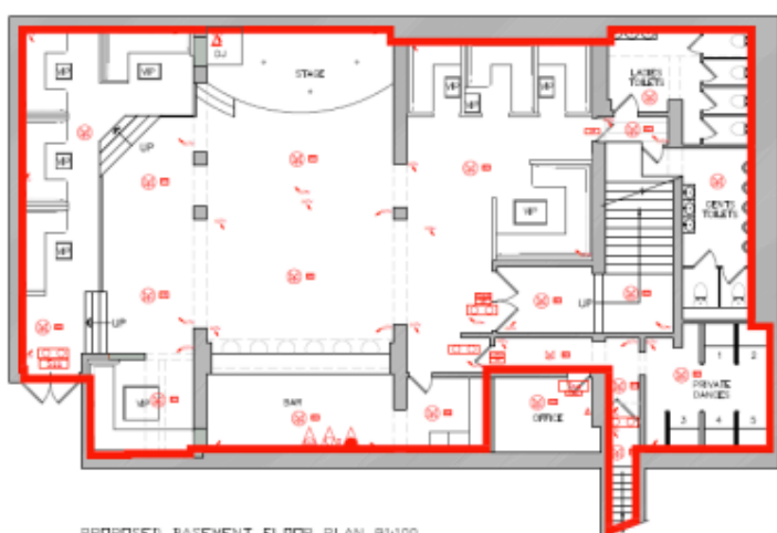
PROPOSED BASEMENT FLOOR PLAN @1:100
